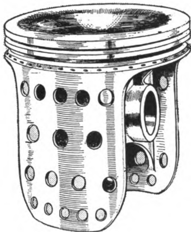
A unique form of piston in which the skirt consists of two perforated slippers
